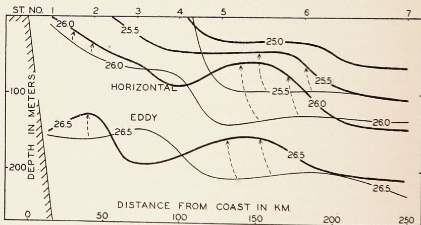
Figure 65. Vertical distribution of density ( \sigma_t ) on cruise II (thin lines) and III (heavy lines). Arrows indicate types of motion which have brought about the changes in the distribution.
